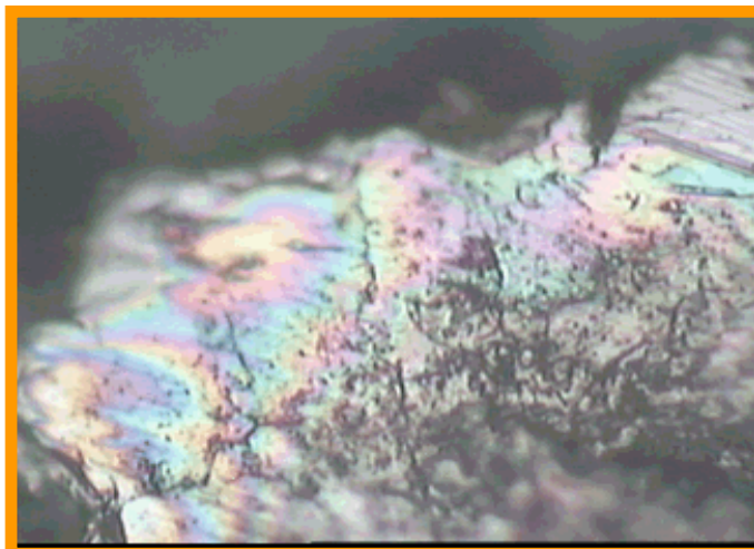
ROLLING CONTACT WEAR (tempering problem): Particles applied to substrate by Syringe Applicator & REO-1 Instrument (as seen through FERRO-VIEW BX40)
